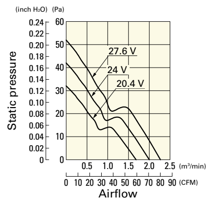
9G1224F401 With pulse sensor
